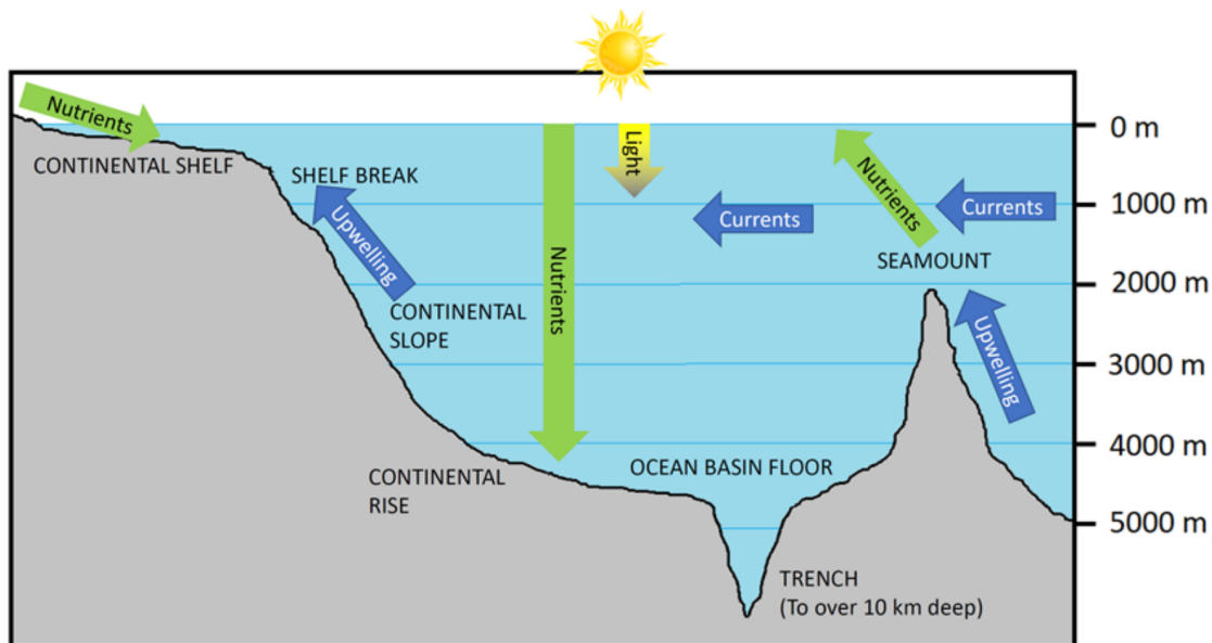
Figure 2. Nutrients fall to light-poor depths, runoff from land and are brought to the surface by currents
